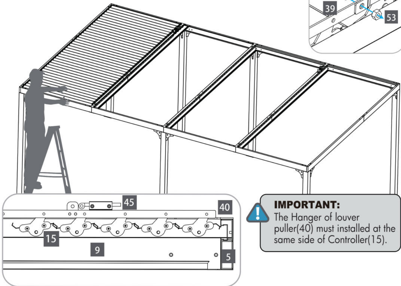
PERSPECTIVE VIEW
