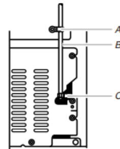
A. Tube clamp B. Copper or PEX tubing C. Compression nut
